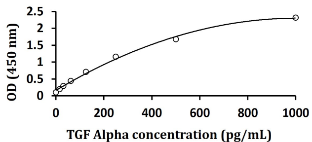
ARG83155 Monkey TGF Alpha ELISA Kit standard curve image
