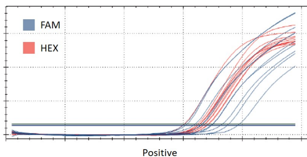
ARG83104 Mycoplasma DNA Detection Kit Standard curve (Positive)
