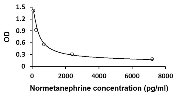
ARG82791 Human 2-MET (Metanephrine + Normetanephrine) ELISA Kit standard curve image
