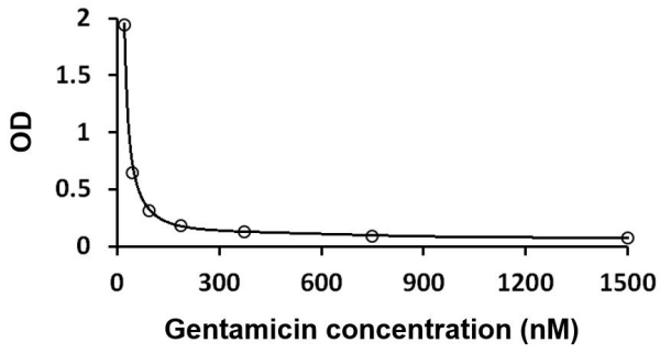
ARG82660 Gentamicin ELISA Kit standard curve image
