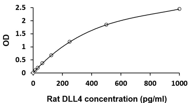
ARG82357 Rat DLL4 ELISA Kit standard curve image
