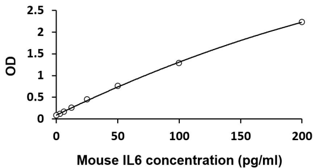
ARG82294 Mouse IL6 (High sensitive) ELISA Kit standard curve image
