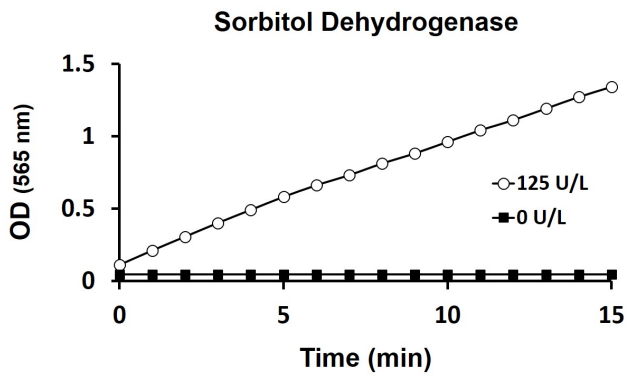
ARG82192 Sorbitol Dehydrogenase Activity Assay Kit (Colorimetric) enzyme kinetics graph
