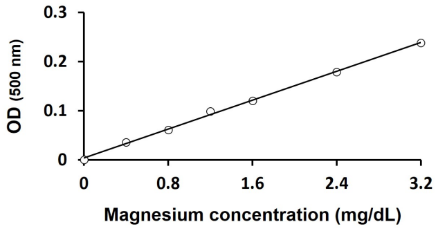
ARG82177 Magnesium Assay Kit (Colorimetric) typical data demonstration image
