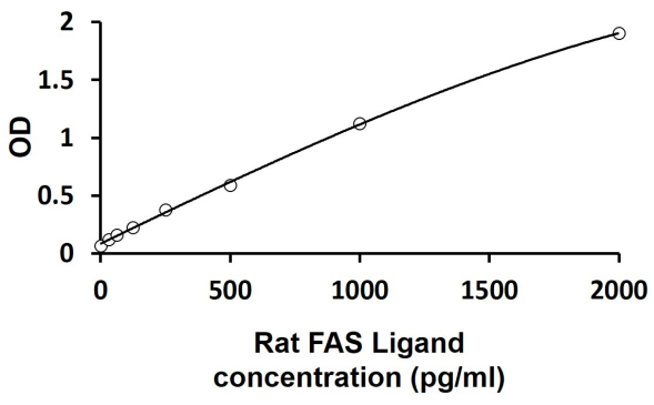
ARG81810 Rat FAS Ligand ELISA Kit standard curve image
