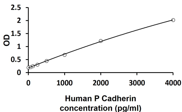
ARG81700 Human P Cadherin ELISA Kit standard curve image
