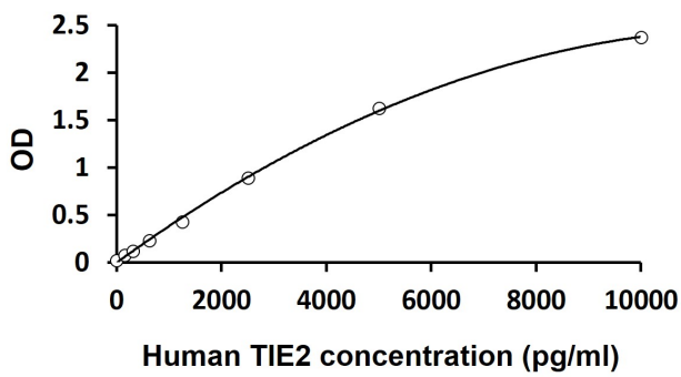
ARG81419 Human TIE2 ELISA Kit standard curve image
