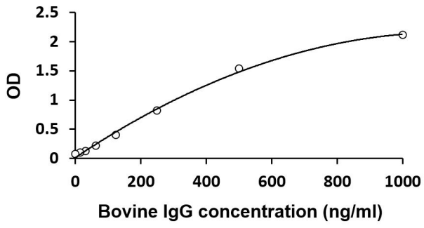
ARG81168 Bovine IgG ELISA Kit standard curve image
