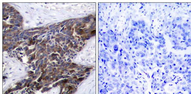
ARG51744 anti-Connexin 43 phospho (Ser367) antibody IHC-P image
